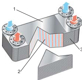
Figure 2. Function: Cover plate (1), Bonded corrugated plates (2) and Bonded seal (3).
