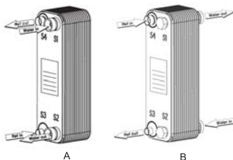
Figure 4. Installation as evaporator (A) and condenser (B).
